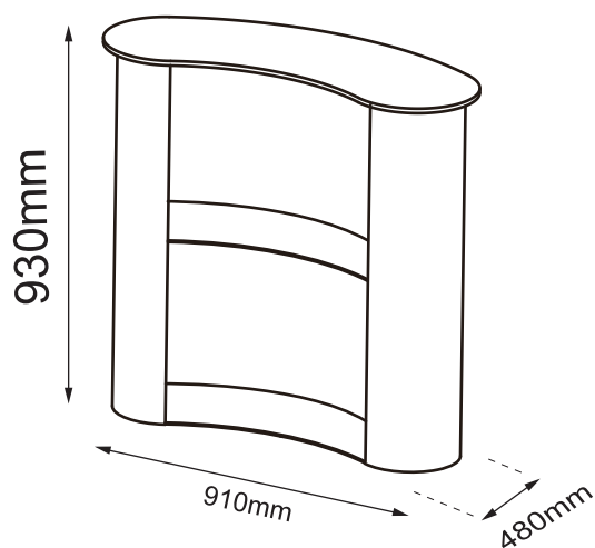
SHELF OPTION
